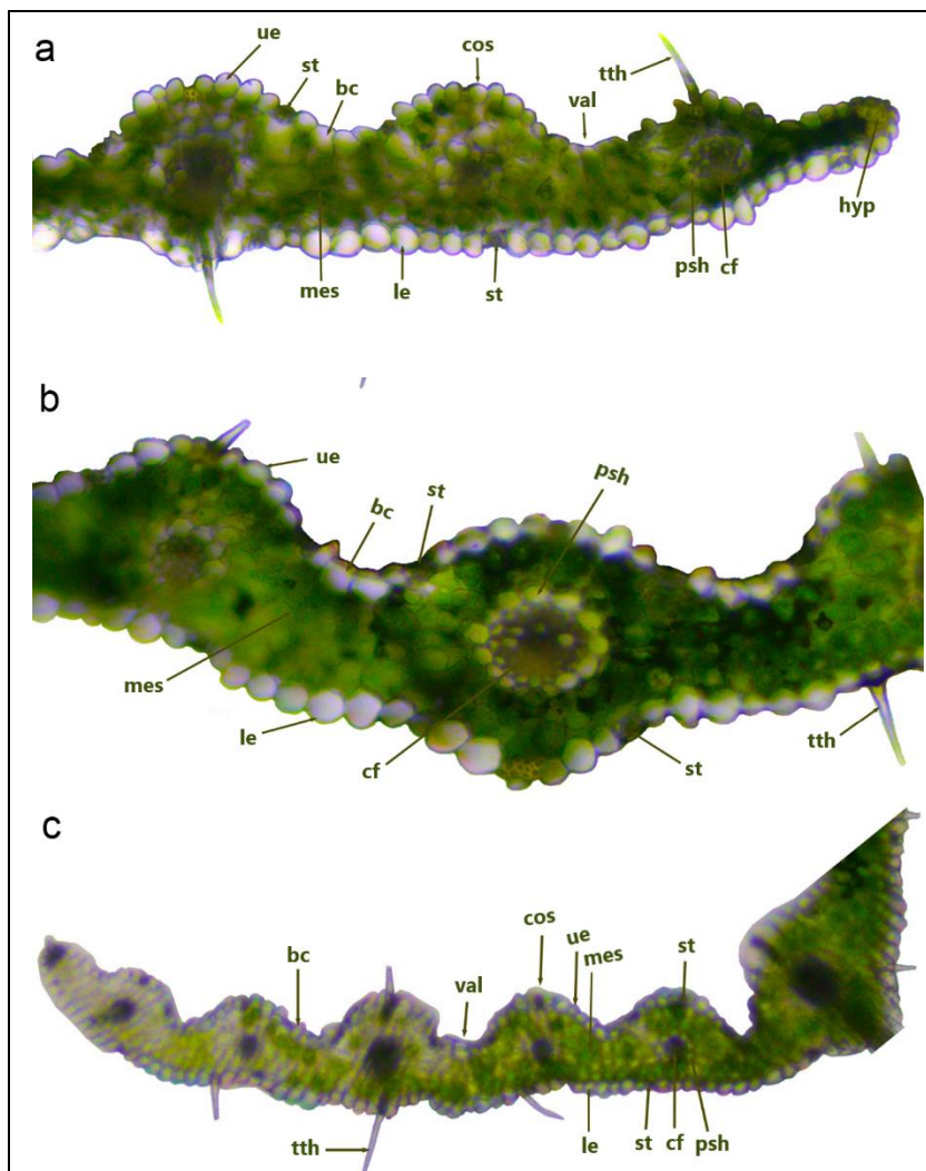
Figure 3. Leaf section
