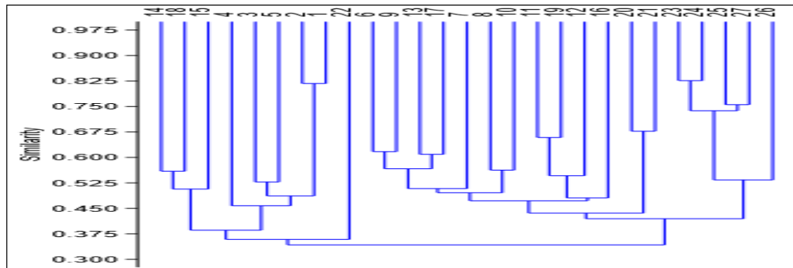
Figure 1. Kulczynski Similarity index of the Agrostio-Festucetum valesiaca association for the northwestern Romania territories
