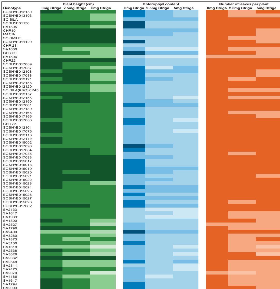
Figure 1. Heatmap analysis for plant height, chlorophyll content and number of leaves per plant for 75 sorghum genotypes exposed to Striga
